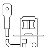
H3 - PK22s
